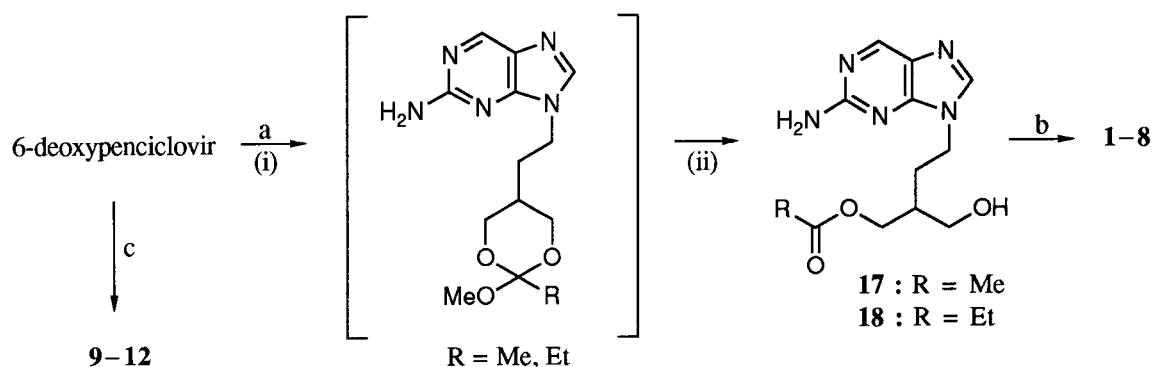
Scheme 2. (a) (i) Trimethyl orthoacetate or triethyl orthopropionate (1.2 equiv), p -TsOH·H 2 O (0.1 equiv), DMF, rt, 2 h; (ii) H 2 O, 1 h; (b) methyl, ethyl, n -propyl, or isopropyl 4-nitrophenyl carbonate (1.2 equiv), DMAP (0.1 equiv), pyridine, 80°C, 20 h; (c) methyl, ethyl, n -propyl, or isopropyl 4-nitrophenyl carbonate (2.1 equiv), DMAP (0.1 equiv), pyridine, 80°C, 24 h.
