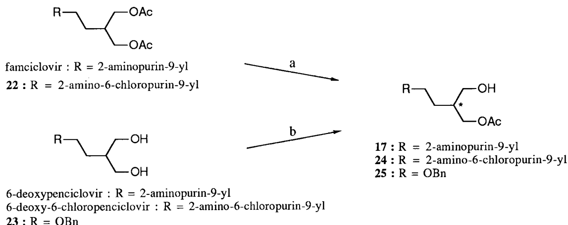
Scheme 4. (a) Lipase (PPL, PFL or CAL), sodium phosphate buffer (pH 7.0), rt; (b) lipase (PPL, PFL or CAL), vinyl acetate, acetone or toluene, rt.
