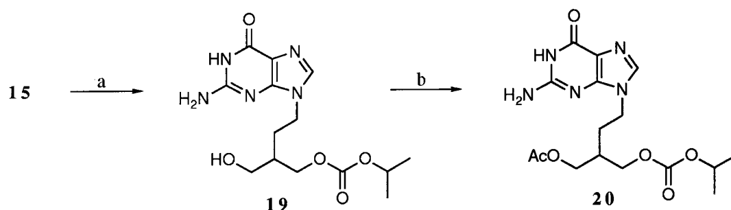
Scheme 3. (a) Adenosine deaminase (10% by wt), phosphate buffer (pH 7.5), rt, 5 days; (b) acetic anhydride (2 equiv), DMAP (0.1 equiv), rt, 1 h.
