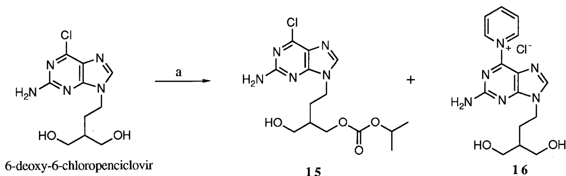
Scheme 1. (a) Isopropyl chloroformate (1.1 equiv), pyridine, 0°C to rt.
